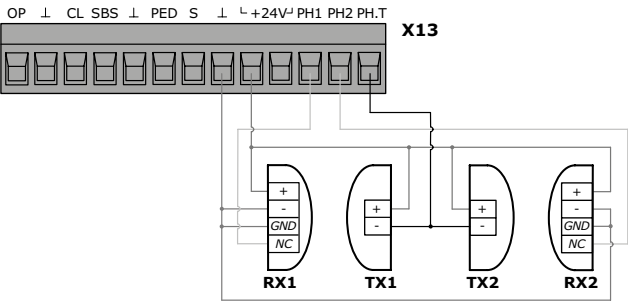
Figure 20. Connecting safety devices ( photocells ) for automatic testing of their operation ( Phototest ) TX1 and RX1 —transmitter and receiver for safe closing photocells; TX2 and RX2 —transmitter and receiver for safe opening photocells
